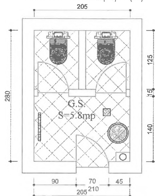
G.S. Parter - Investitii propus (16)
